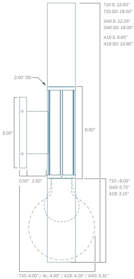
RPD14DS: Side view - seen here with two T10 bulbs (A19 and G40 in dashed lines).
