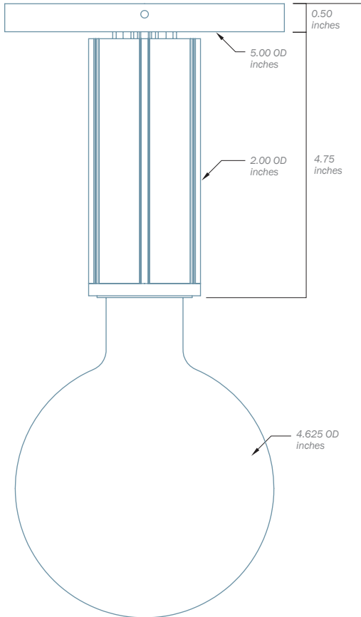
RPD14C: Side view - seen here with a G40 bulb
