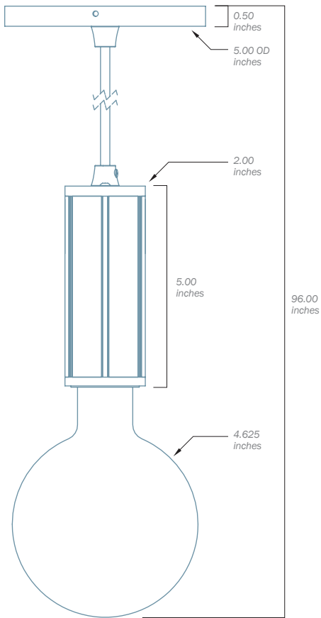
RPD14P: Side view - seen here with a G40 bulb
